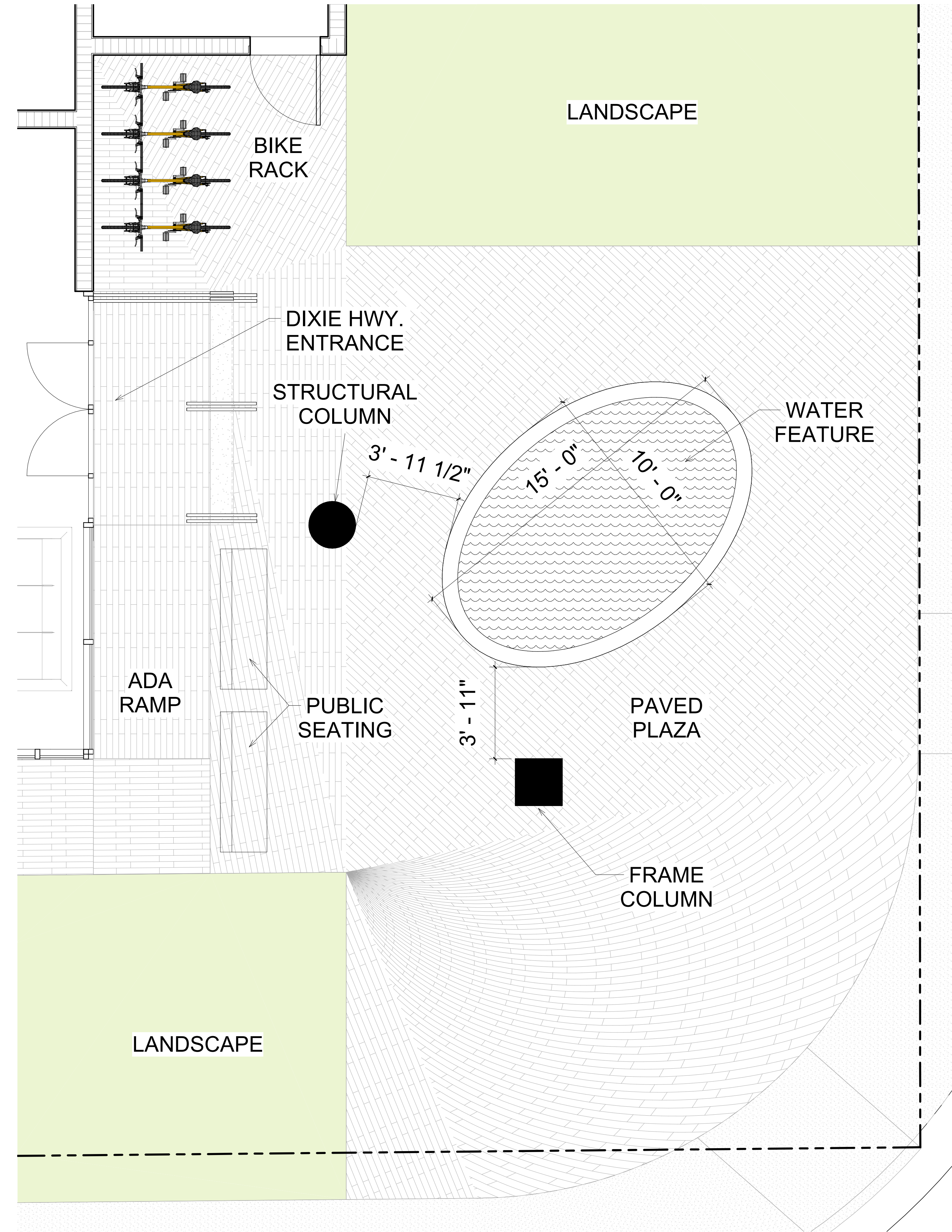
1 | WATER FEATURE SCALE: 3/8" = 1'-0"
