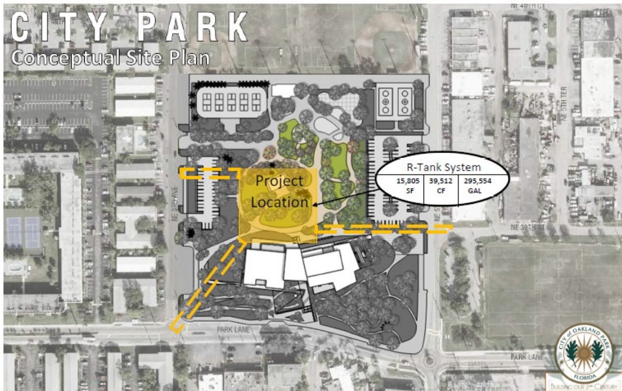
Figure 1. Proposed City Park Stormwater Capture and Reuse Project
